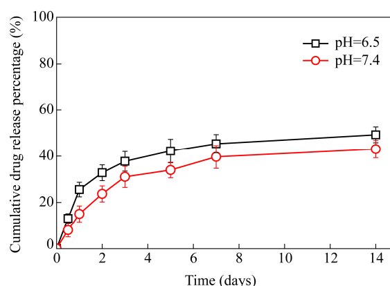
Fig. 2 In vitro drug release of PLGA microparticles with internal pores at different pH values
